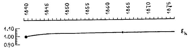
Fig. 1. Curve for the value of \epsilon_h used in the final reduction of the eye-readings for the interval 1843—76.
