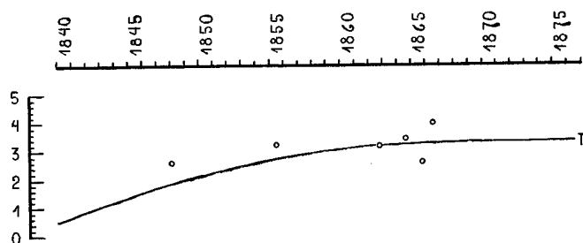
Fig. 3. Curve for the value of \lambda actually used in the final reduction of the eye-readings for the interval 1843—76.
